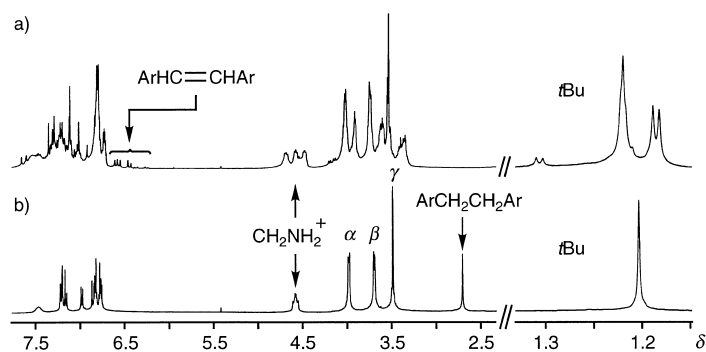
Figure 5. Partial ^1\text{H} NMR spectra (400 MHz, \text{CD}_3\text{CN} , 298 K) of a) the E/Z isomer mixture of [4]rotaxanes 15a-3H·3PF 6 and b) the hydrogenated [4]rotaxane 16a-3H·3PF 6 .
