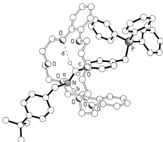
Figure 2. The cationic portion of the solid-state structure of the [2]rotaxane 2a-H ·2PF 6 . The hydrogen bonding geometries, X···O, H···O [Å], and X–H···O [°]: a) 3.05, 2.21, 156; b) 3.14, 2.30, 154; c) 3.27, 2.40, 150; d) 3.23, 2.34, 153.
