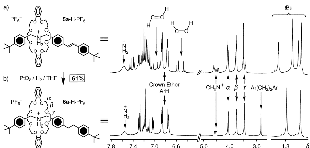
Figure 4. Partial ^1\text{H} NMR spectra (400 MHz, \text{CD}_3\text{CN} , 298 K) of a) the E/Z isomer mixture of [2]rotaxanes 5a-H · \text{PF}_6 and b) the hydrogenated [2]rotaxane 6a-H · \text{PF}_6 .
