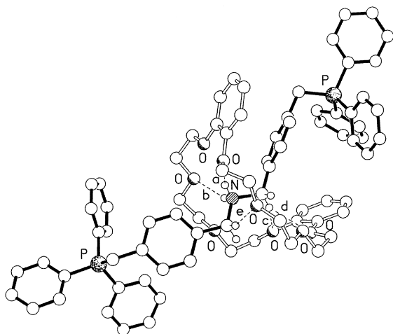
Figure 3. The cationic portion of the solid-state structure of the [2]rotaxane 4a-H · 3PF 6 . The hydrogen bonding geometries, X···O, H···O [Å], and X–H···O [°]: a) 3.05, 2.26, 147; b) 2.96, 2.15, 151; c) 3.33, 2.44, 153; d) 3.21, 2.41, 156; e) 3.22, 2.33, 156.
