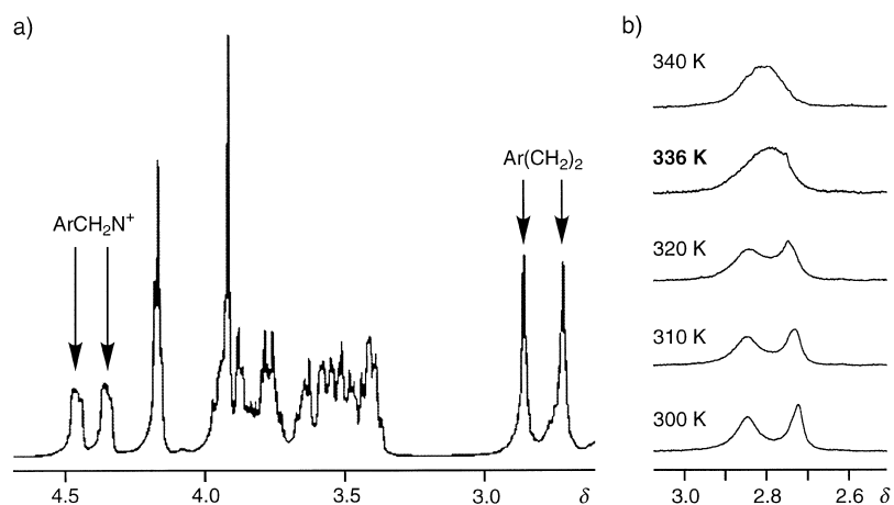
Figure 6. a) Partial 1 H NMR spectrum (400 MHz, CD 3 CN, 298 K) of the two-station molecular shuttle 17b ·2H·2PF 6 depicting the asymmetrical nature of the shuttle at ambient temperature. b) Partial variable temperature 1 H NMR spectra (400 MHz, CD 3 OD) of molecular shuttle 17b ·2H·2PF 6 highlighting the signals of the Ar-CH 2 CH 2 -Ar groups, which coalesce at 336 K.
