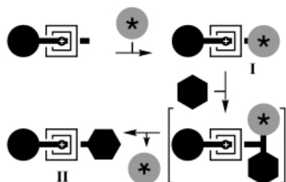
Figure 1. Graphical representation of the threading-followed-by-stoppering approach to [2]rotaxanes and the subsequent stopper-exchange concept.
